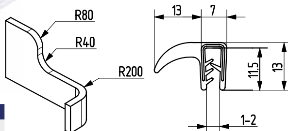
Part no. Material 90GU-E06-00 EPDM
