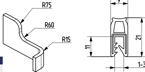
Part no. Material 90GU-E20-00 EPDM/PVC
